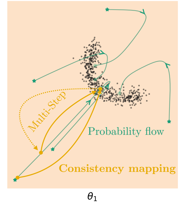
Consistency Models
